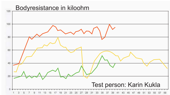
The red graph show the high body resistance of the test person, caused by the geologically disturbed areas.
